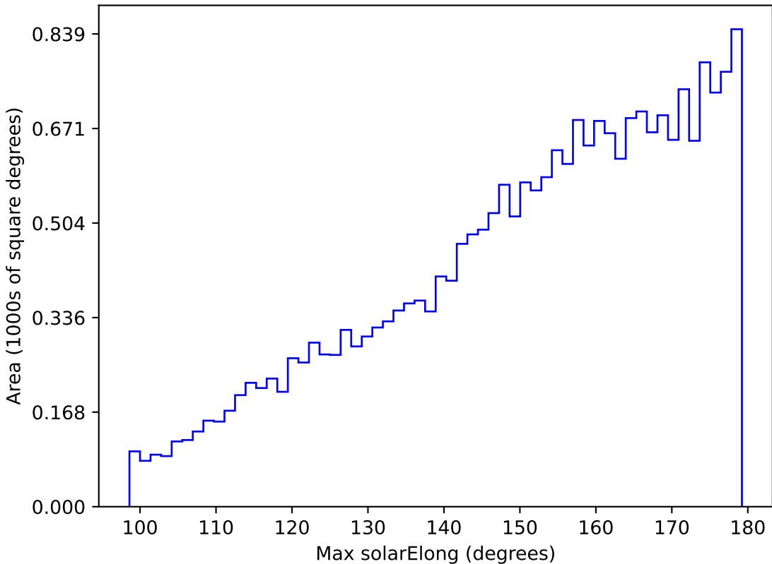
noroll_mjdp270_v3.4_10yrs All sky y band: Max solarElong
