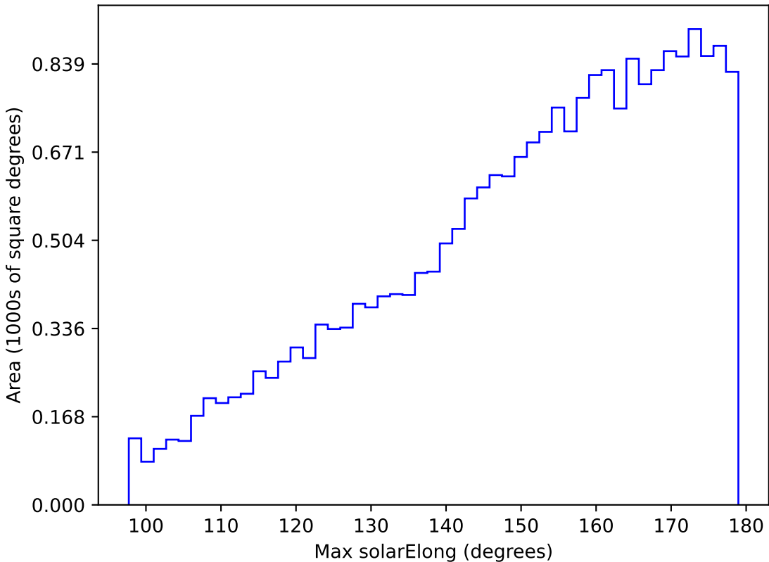
noroll_mjdp270_v3.4_10yrs All sky u band: Max solarElong
