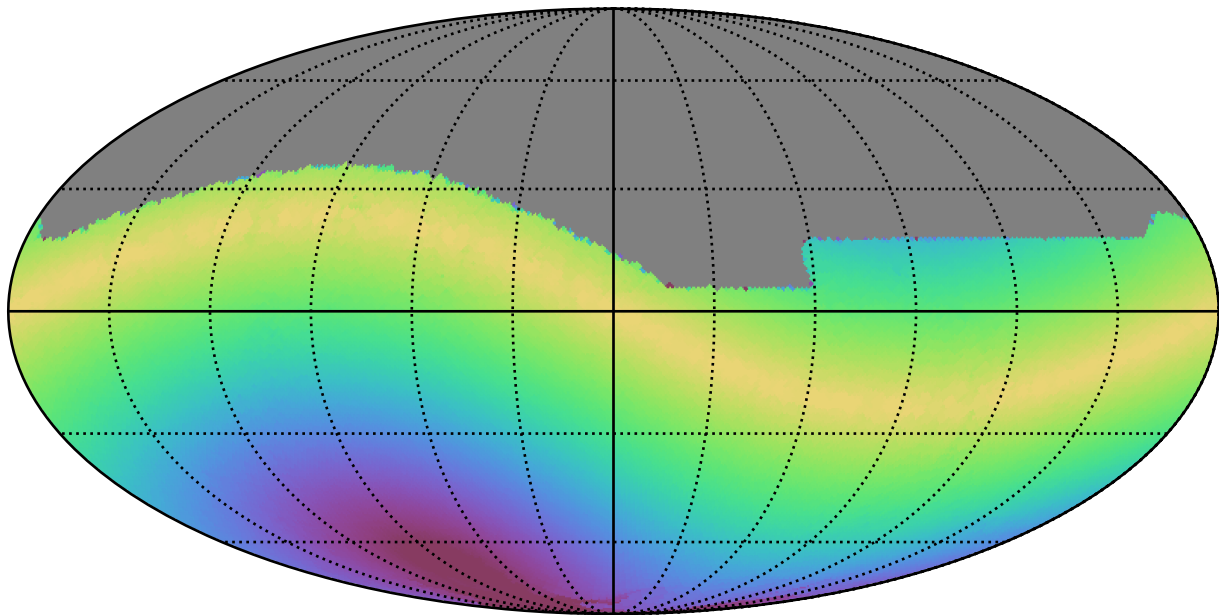
noroll_mjdp270_v3.4_10yrs All sky r band: Max solarElong
