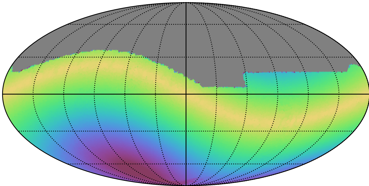
noroll_mjdp270_v3.4_10yrs All sky i band: Max solarElong
