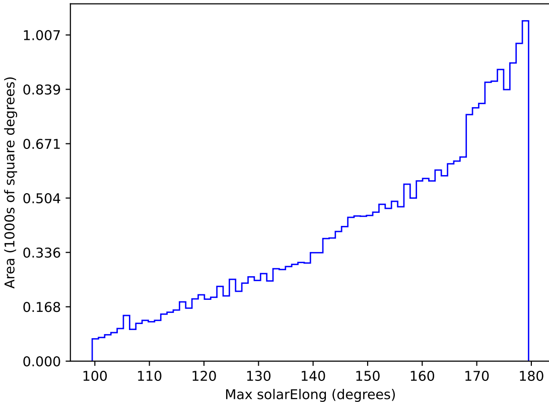
noroll_mjdp270_v3.4_10yrs All sky i band: Max solarElong
