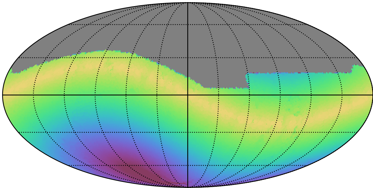
noroll_mjdp270_v3.4_10yrs All sky g band: Max solarElong
