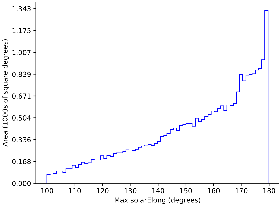
noroll_mjdp270_v3.4_10yrs All sky all bands: Max solarElong
