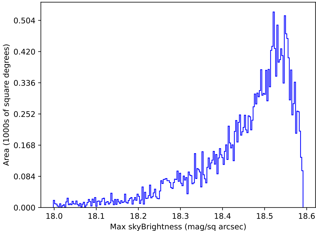
noroll_mjdp270_v3.4_10yrs Yr 1 y band: Max skyBrightness
