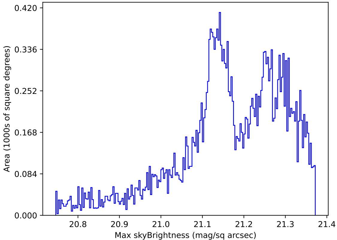
noroll_mjdp270_v3.4_10yrs Yr 1 r band: Max skyBrightness
