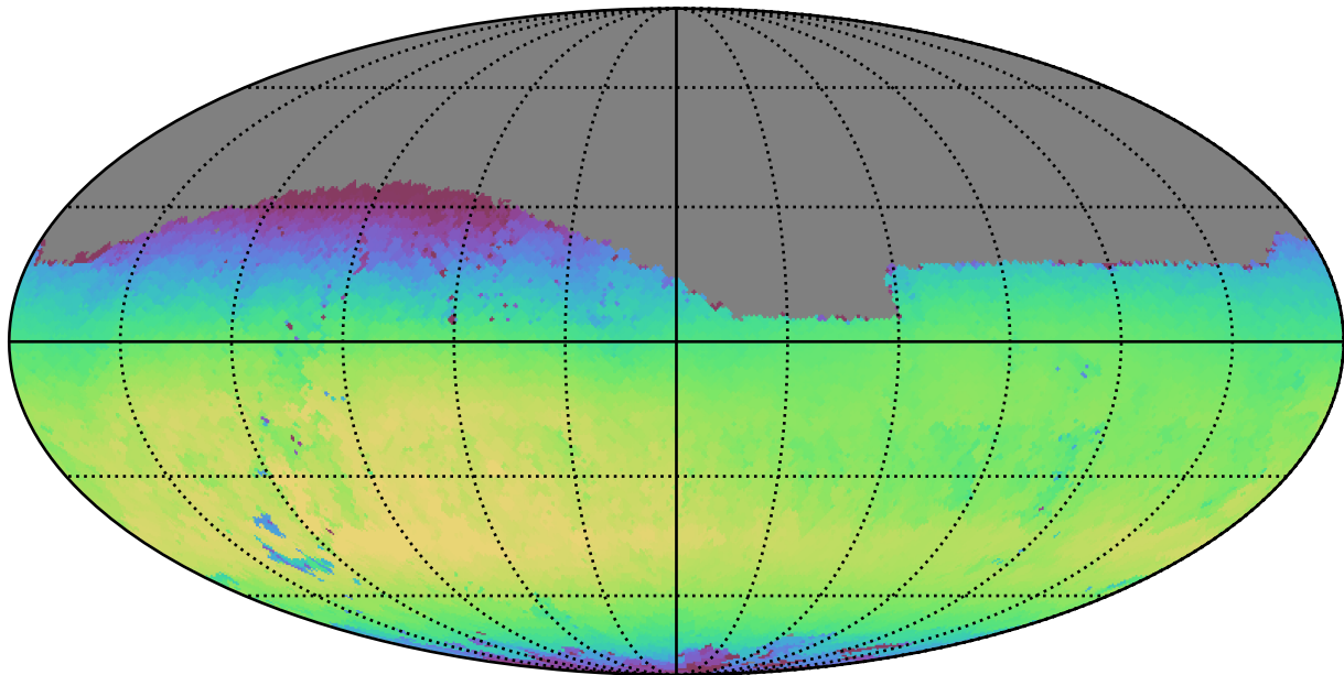
noroll_mjdp270_v3.4_10yrs Yr 1 i band: Max skyBrightness
