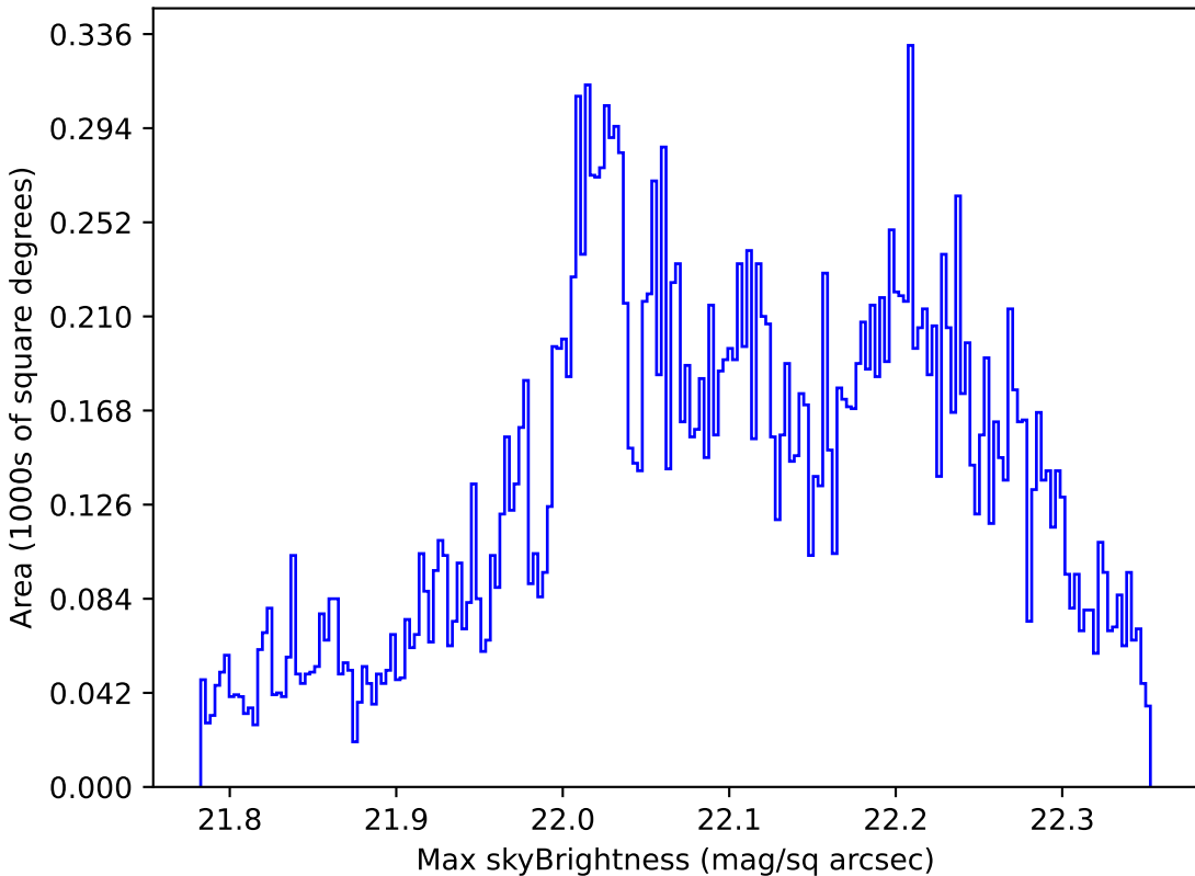
noroll_mjdp270_v3.4_10yrs Yr 1 g band: Max skyBrightness
