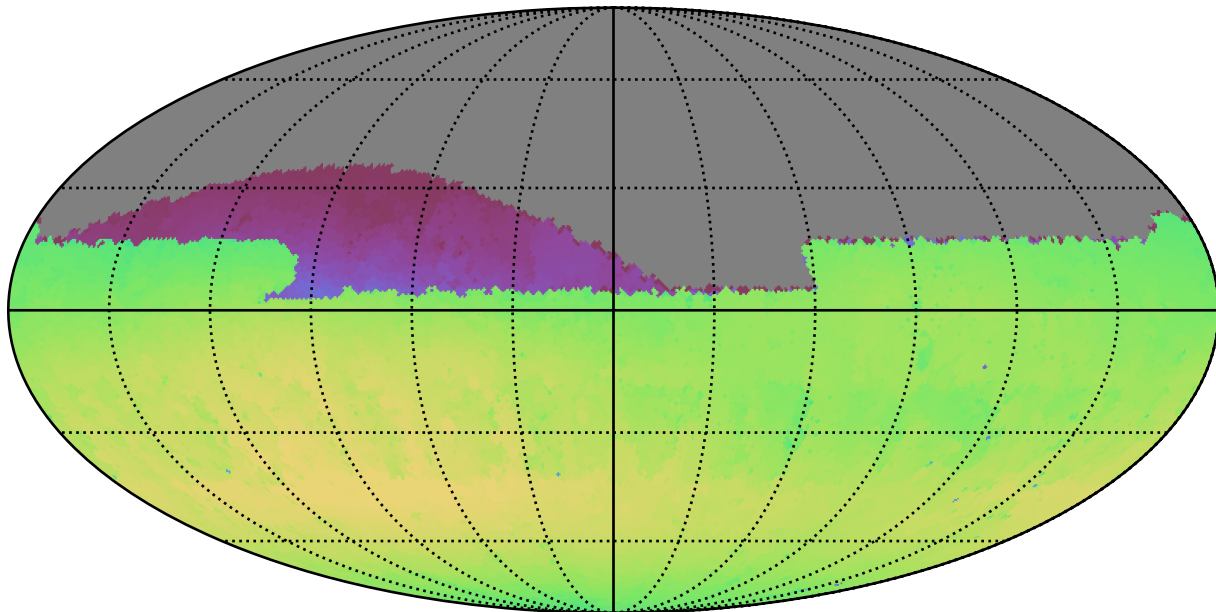
noroll_mjdp270_v3.4_10yrs Yr 1 all bands: Max skyBrightness
