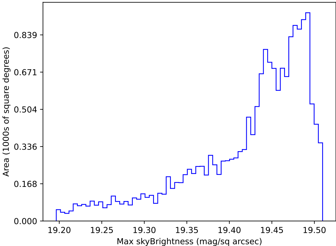
noroll_mjdp270_v3.4_10yrs WFD z band: Max skyBrightness
