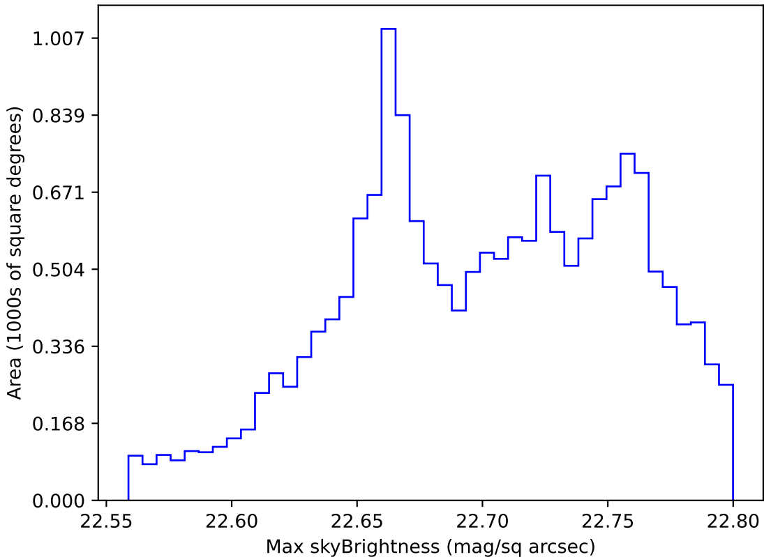
noroll_mjdp270_v3.4_10yrs WFD u band: Max skyBrightness
