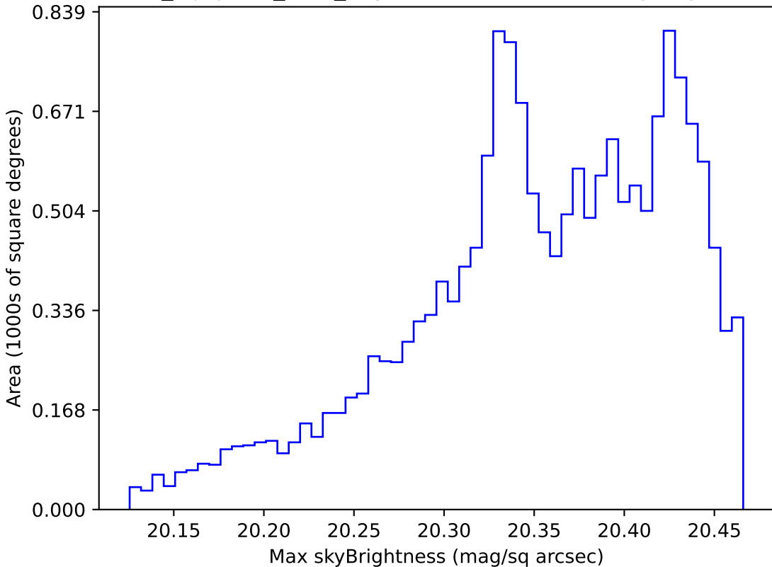
noroll_mjdp270_v3.4_10yrs WFD i band: Max skyBrightness
