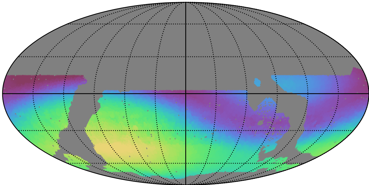
noroll_mjdp270_v3.4_10yrs WFD g band: Max skyBrightness
