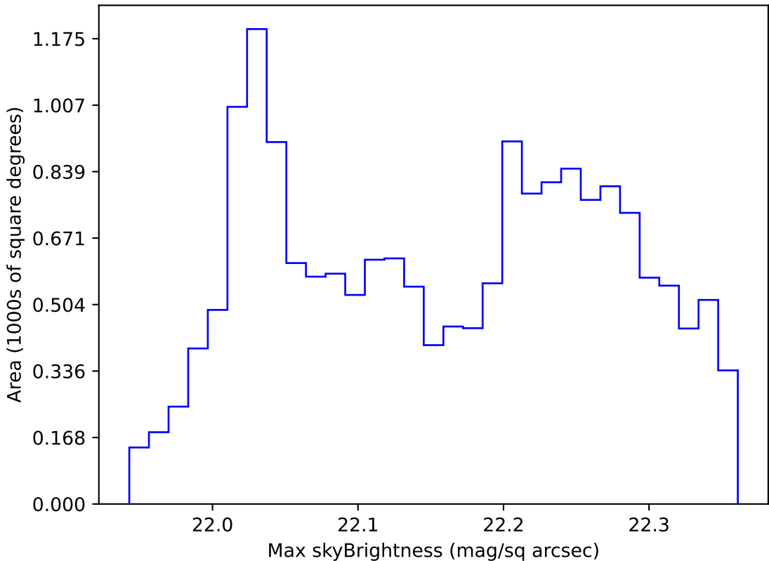
noroll_mjdp270_v3.4_10yrs WFD g band: Max skyBrightness
