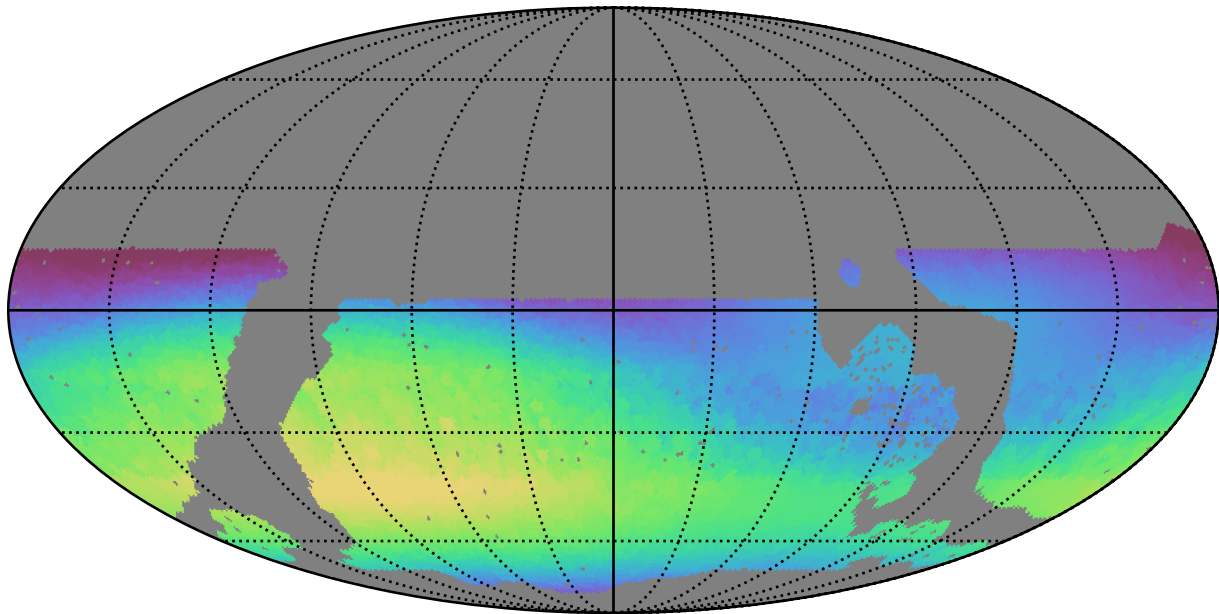
noroll_mjdp270_v3.4_10yrs WFD all bands: Max skyBrightness
