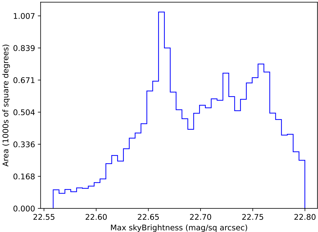
noroll_mjdp270_v3.4_10yrs WFD all bands: Max skyBrightness
