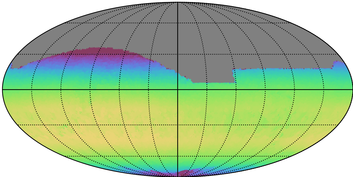
noroll_mjdp270_v3.4_10yrs All sky z band: Max skyBrightness
