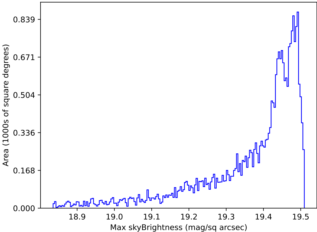
noroll_mjdp270_v3.4_10yrs All sky z band: Max skyBrightness
