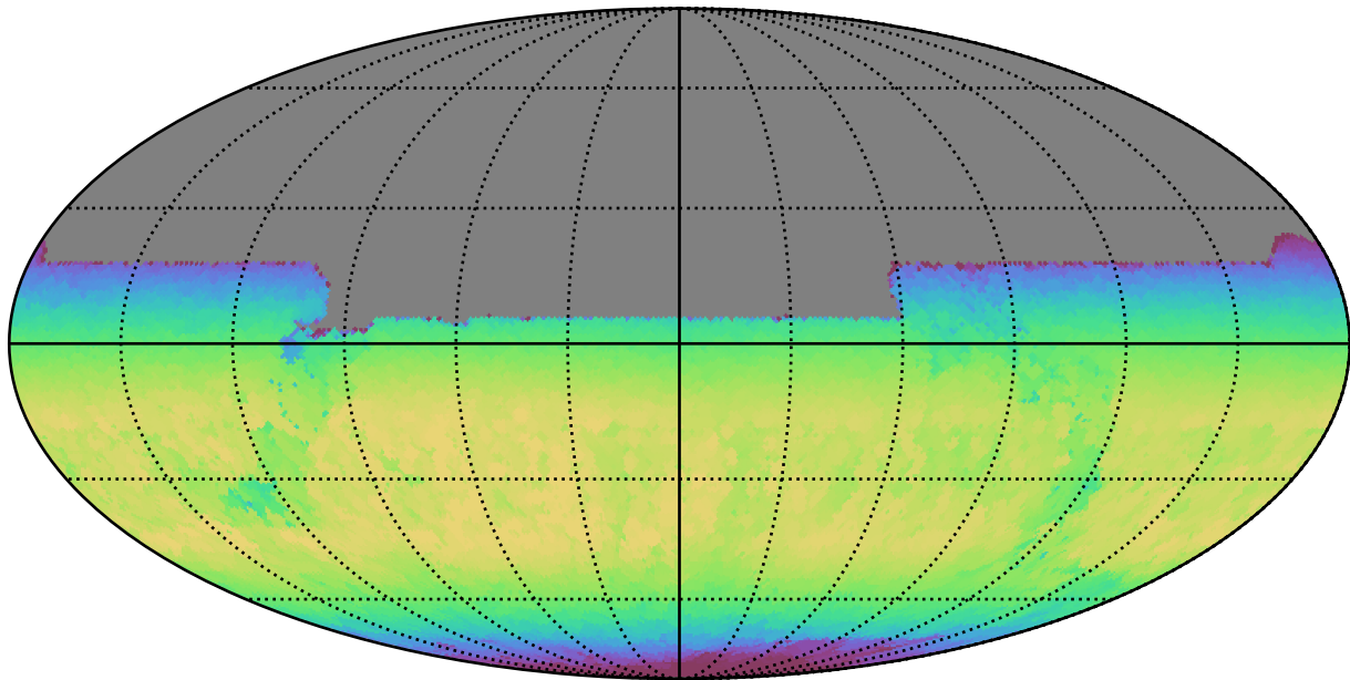
noroll_mjdp270_v3.4_10yrs All sky y band: Max skyBrightness
