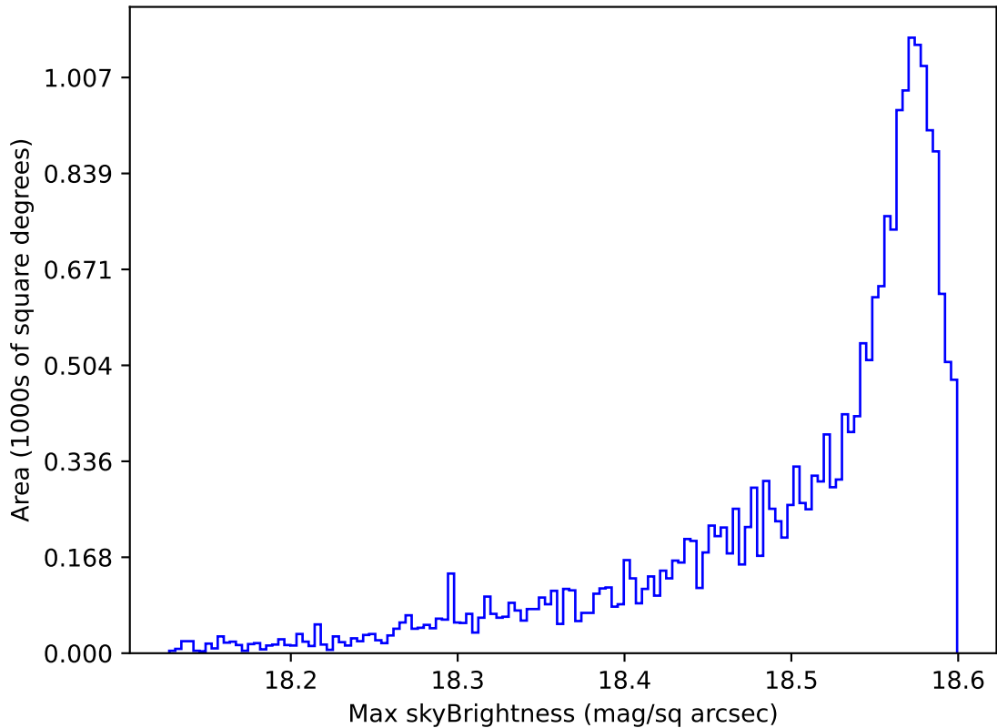
noroll_mjdp270_v3.4_10yrs All sky y band: Max skyBrightness
