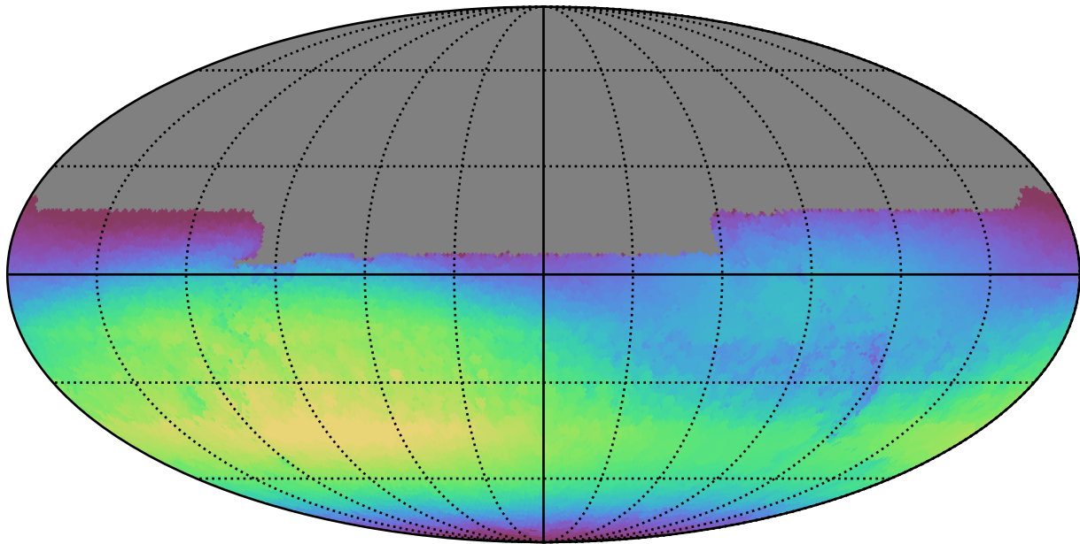
noroll_mjdp270_v3.4_10yrs All sky u band: Max skyBrightness
