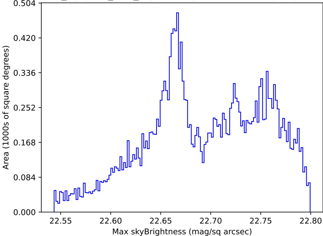
noroll_mjdp270_v3.4_10yrs All sky u band: Max skyBrightness
