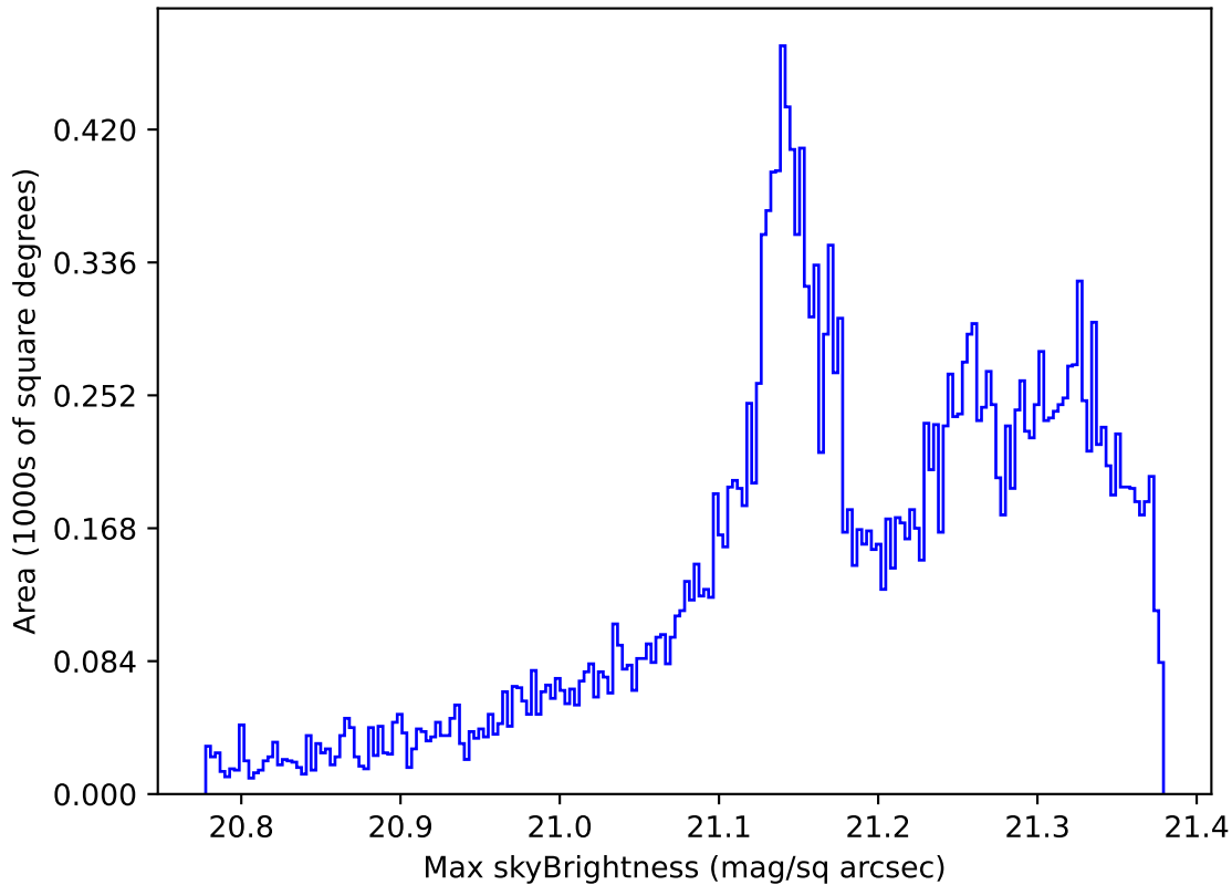
noroll_mjdp270_v3.4_10yrs All sky r band: Max skyBrightness
