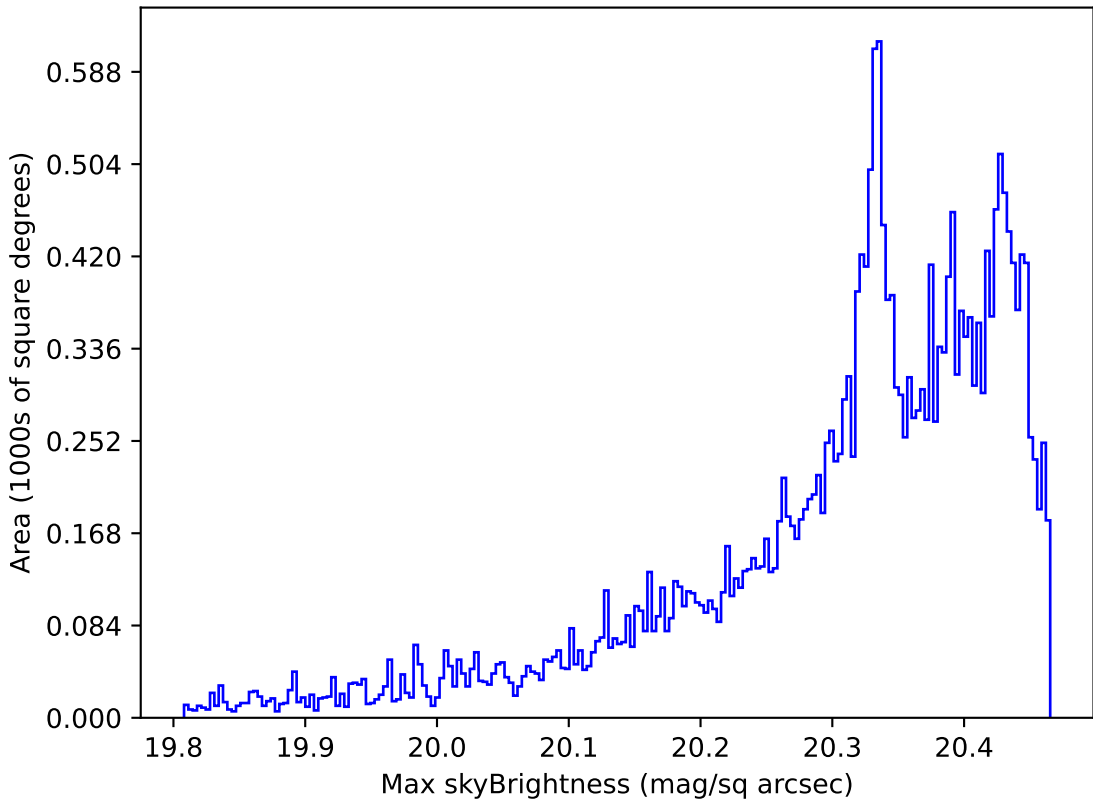
noroll_mjdp270_v3.4_10yrs All sky i band: Max skyBrightness
