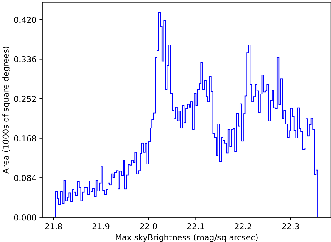
noroll_mjdp270_v3.4_10yrs All sky g band: Max skyBrightness
