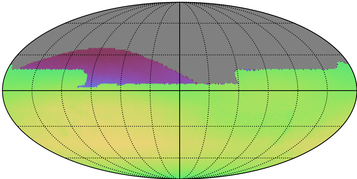
noroll_mjdp270_v3.4_10yrs All sky all bands: Max skyBrightness
