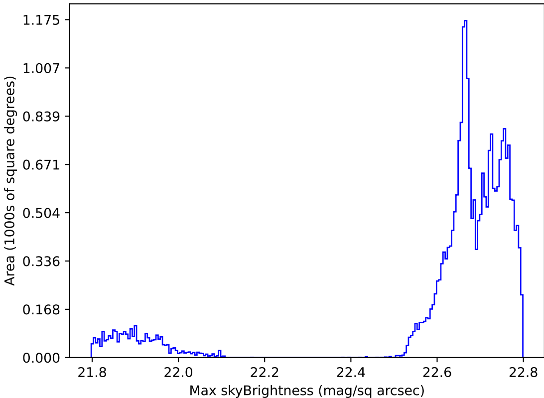
noroll_mjdp270_v3.4_10yrs All sky all bands: Max skyBrightness
