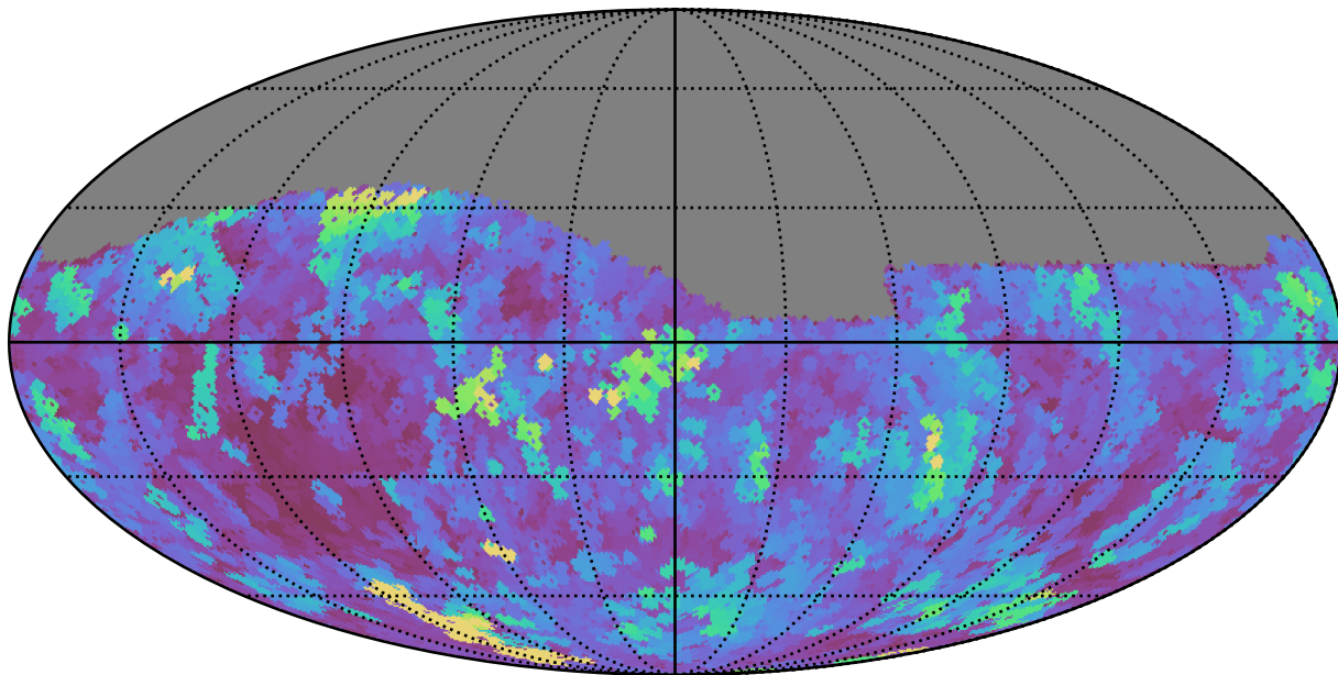
noroll_mjdp270_v3.4_10yrs Yr 1 z band: Max seeingGeom
