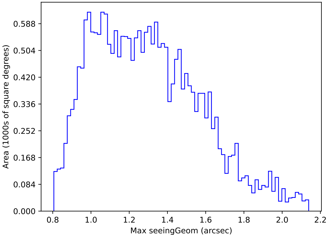
noroll_mjdp270_v3.4_10yrs Yr 1 u band: Max seeingGeom
