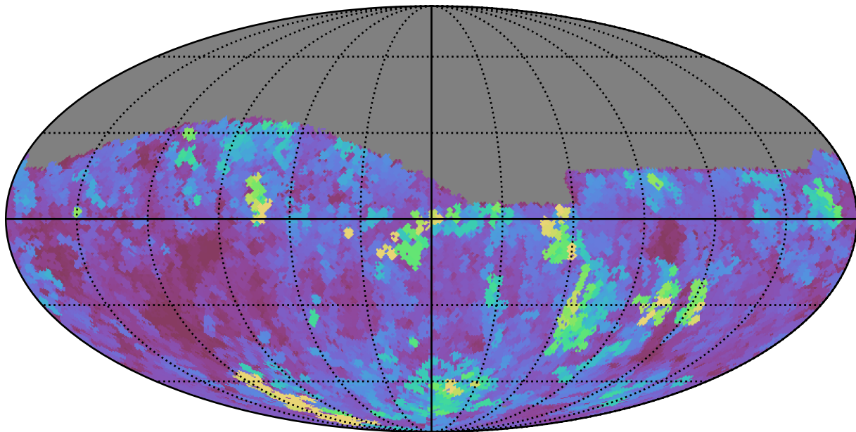
noroll_mjdp270_v3.4_10yrs Yr 1 i band: Max seeingGeom
