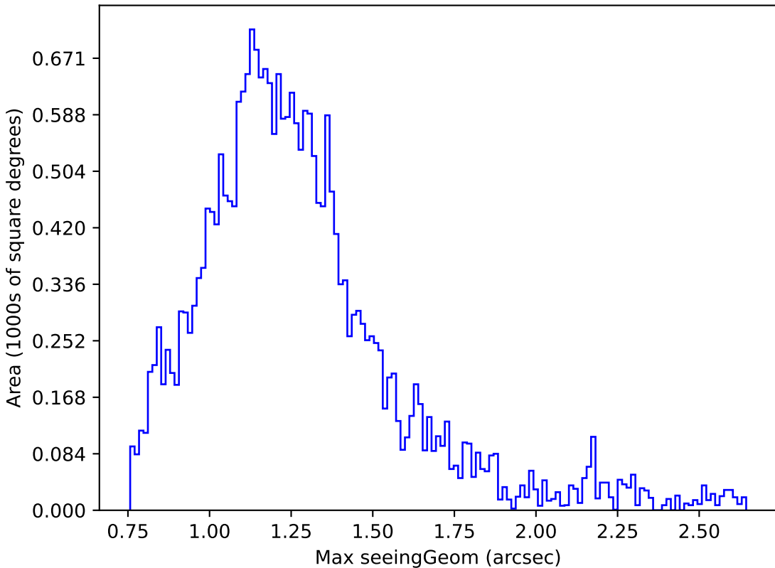
noroll_mjdp270_v3.4_10yrs Yr 1 i band: Max seeingGeom
