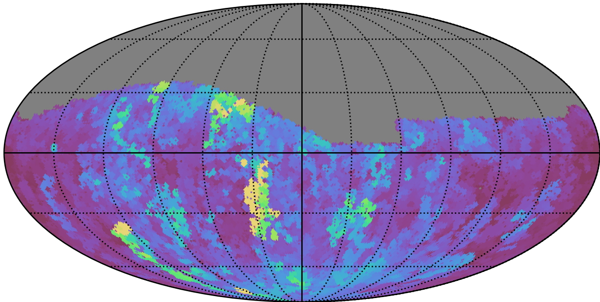
noroll_mjdp270_v3.4_10yrs Yr 1 g band: Max seeingGeom
