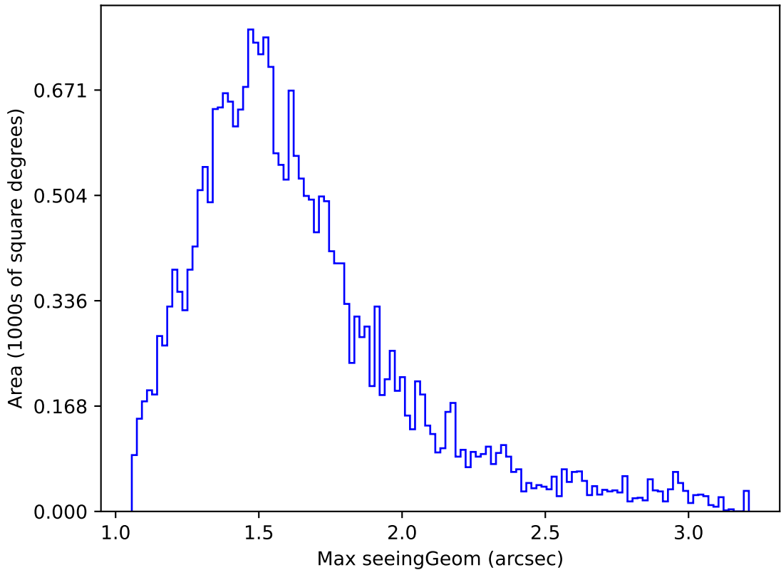
noroll_mjdp270_v3.4_10yrs Yr 1 all bands: Max seeingGeom
