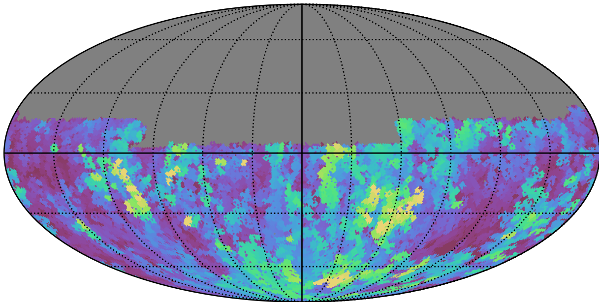
noroll_mjdp270_v3.4_10yrs Yr 1 u band: Max seeingEff
