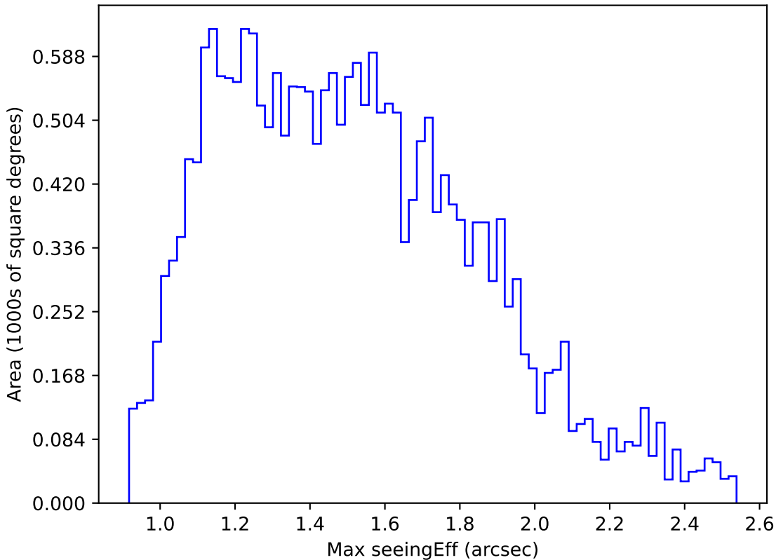
noroll_mjdp270_v3.4_10yrs Yr 1 u band: Max seeingEff
