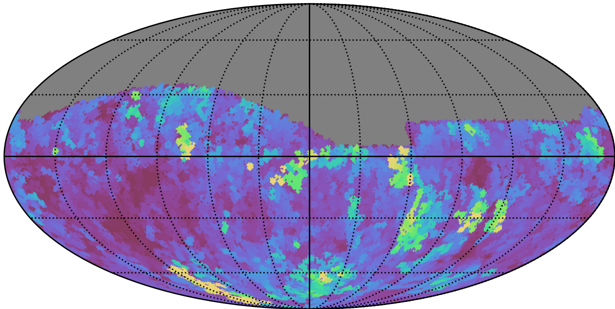
noroll_mjdp270_v3.4_10yrs Yr 1 i band: Max seeingEff
