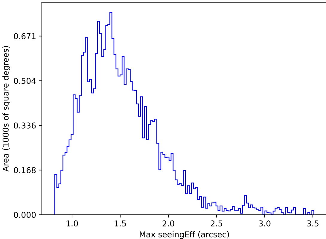
noroll_mjdp270_v3.4_10yrs Yr 1 g band: Max seeingEff
