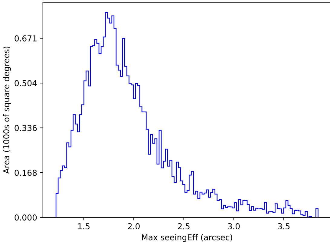
noroll_mjdp270_v3.4_10yrs Yr 1 all bands: Max seeingEff
