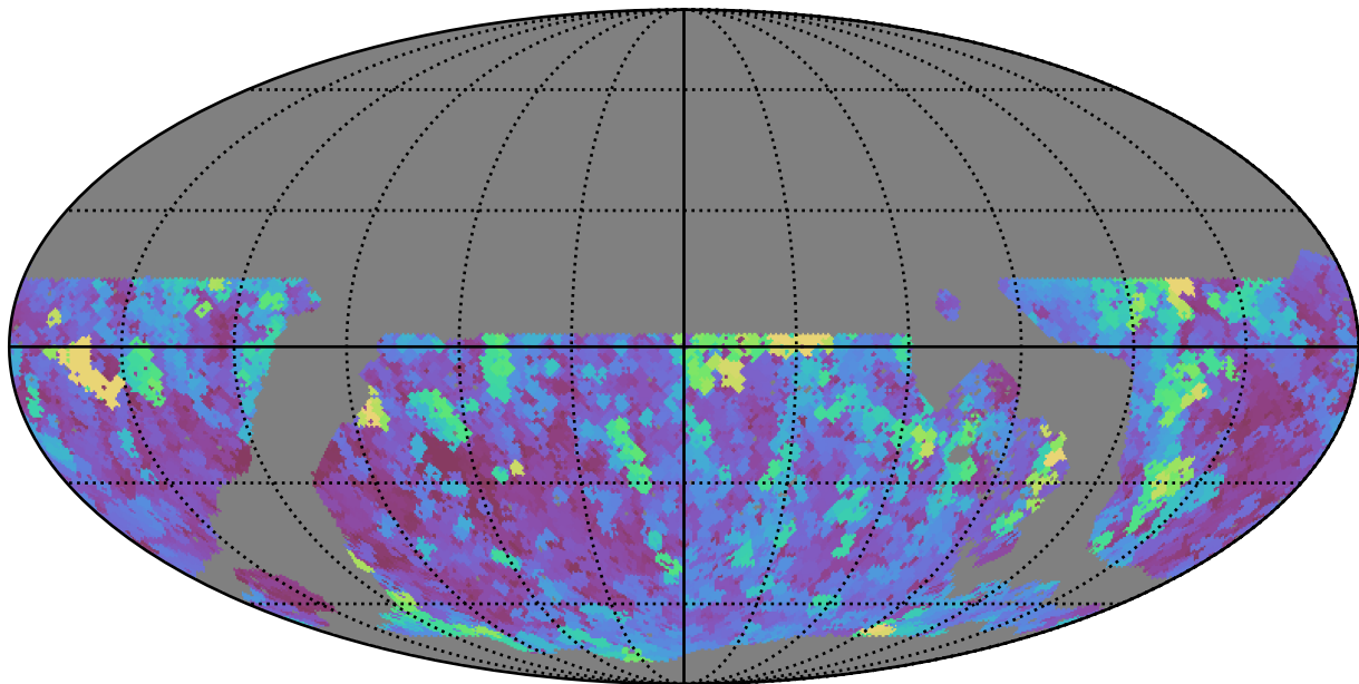
noroll_mjdp270_v3.4_10yrs WFD z band: Max seeingEff
