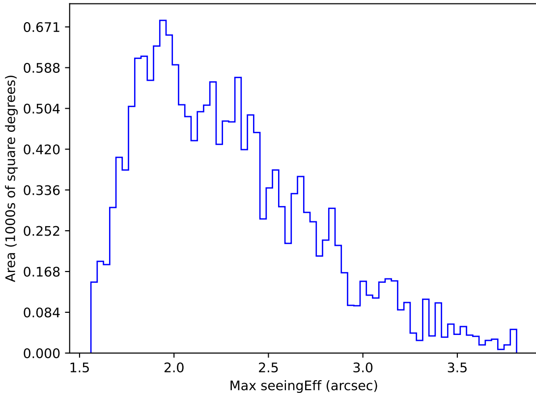
noroll_mjdp270_v3.4_10yrs WFD y band: Max seeingEff
