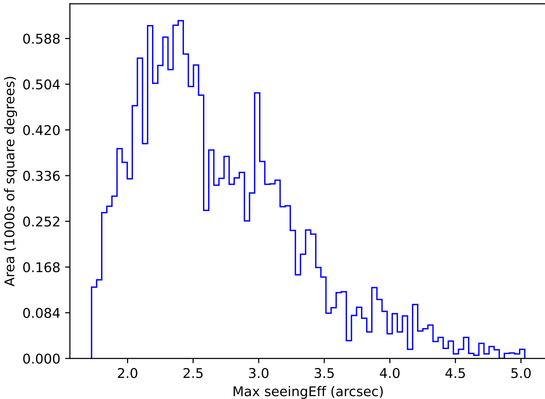
noroll_mjdp270_v3.4_10yrs WFD r band: Max seeingEff
