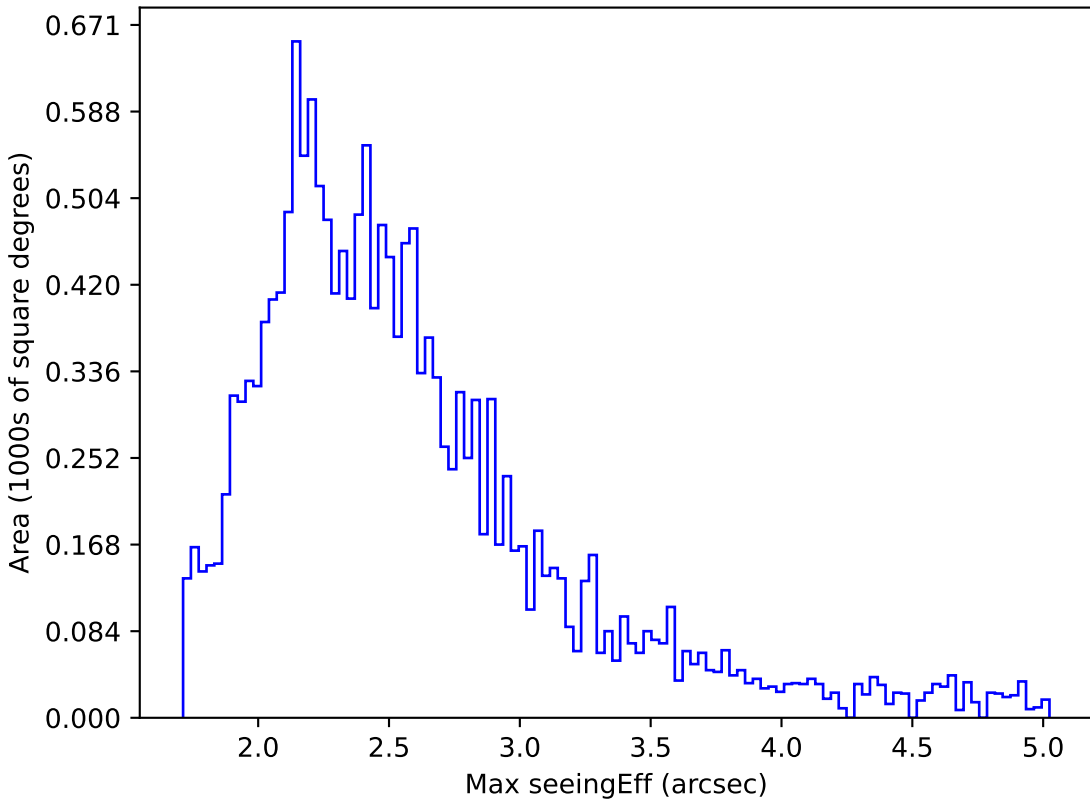
noroll_mjdp270_v3.4_10yrs WFD i band: Max seeingEff
