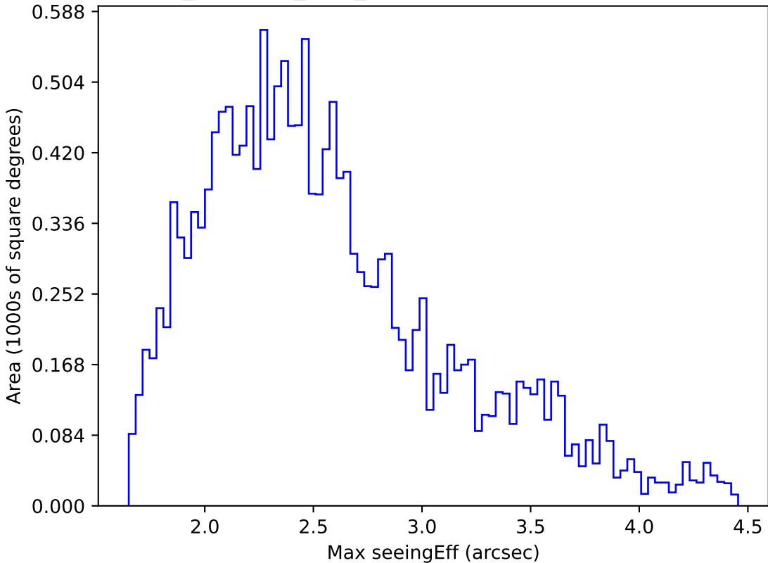
noroll_mjdp270_v3.4_10yrs WFD g band: Max seeingEff
