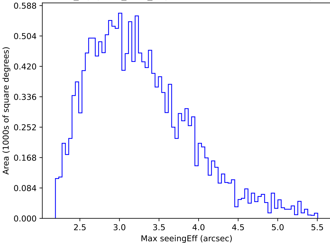
noroll_mjdp270_v3.4_10yrs WFD all bands: Max seeingEff
