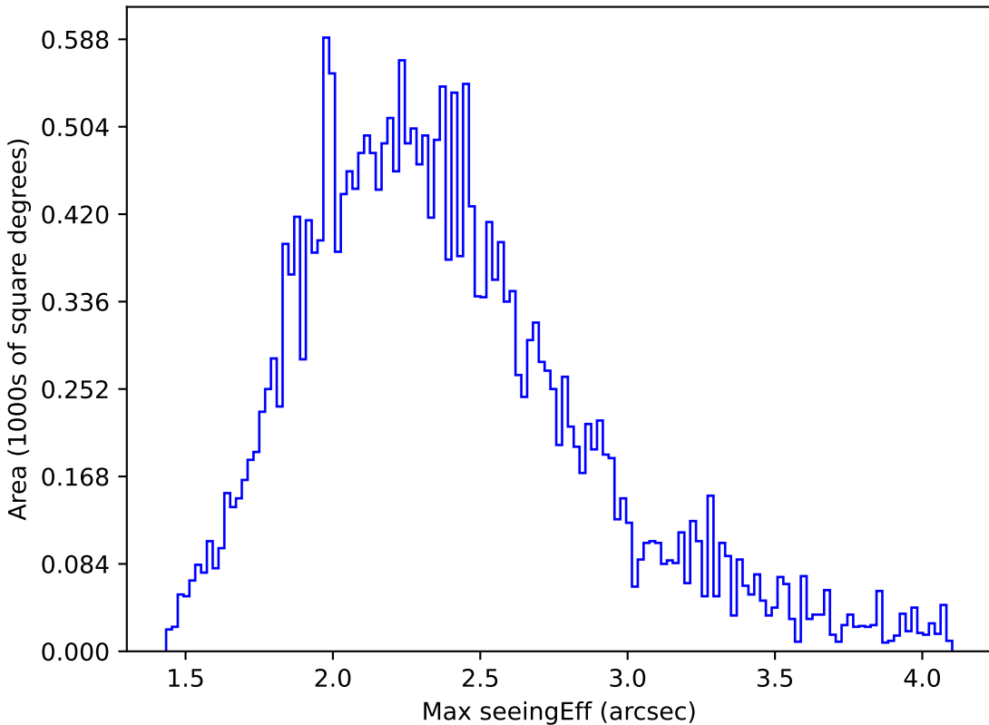
noroll_mjdp270_v3.4_10yrs All sky z band: Max seeingEff
