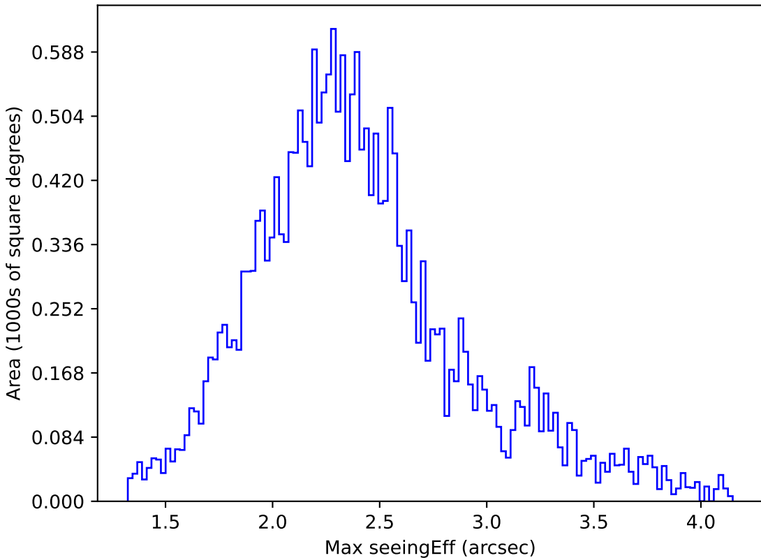
noroll_mjdp270_v3.4_10yrs All sky u band: Max seeingEff
