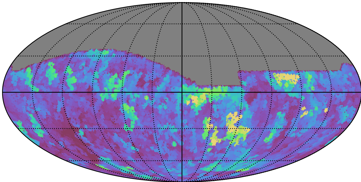
noroll_mjdp270_v3.4_10yrs All sky i band: Max seeingEff
